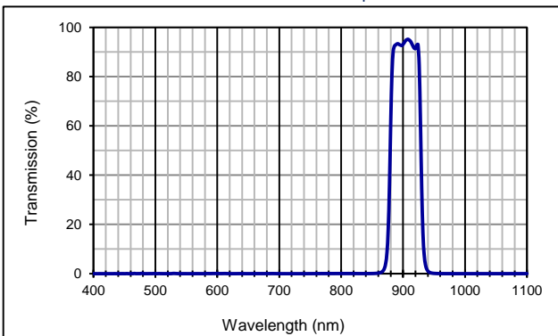
Filter characteristics 905 nm band pass
